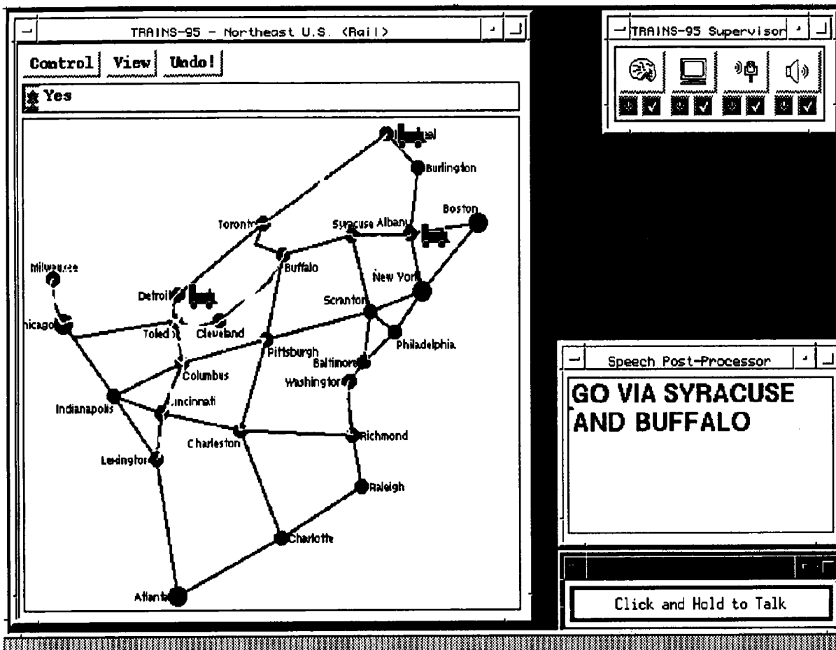
Figure 7: TRAINS User Interface
